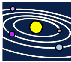
Solar system
