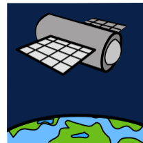
satellite
