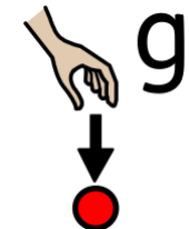
gravity
