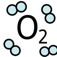
oxygen
